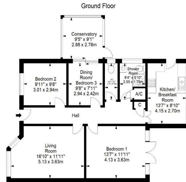
Approximate gross internal floor area 92.1 sq m/ 991.4 sq ft Whilst every care has been taken to ensure accuracy, dimensions are approximate and for illustrative purposes only. All rights reserved.
